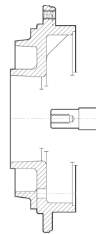
Goulds Motor Adaptor 145JM to 184JM
