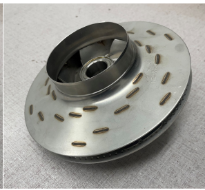
Goulds Stamped Impeller, 5-35/64"
