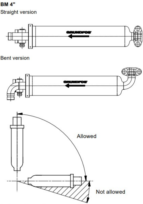
Fig. 1 Positional requirements
