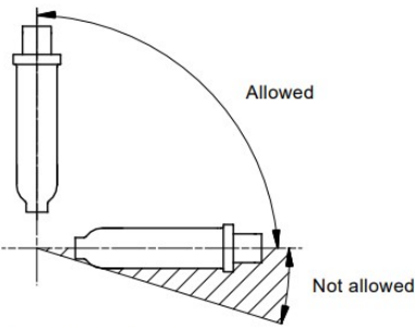
Fig. 1 Positional requirements
