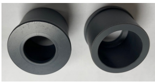
PVC 1" Socket Weld
