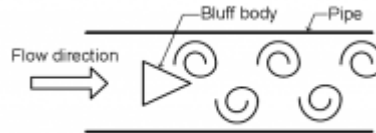
Fig. 2 Operating principle
