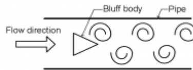
Fig. 2 Operating principle
