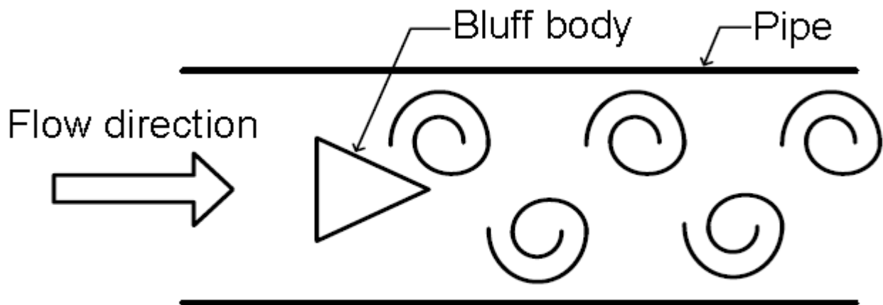
Fig. 2 Operating principle
