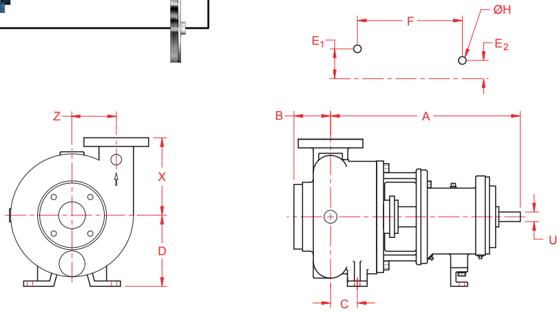
Pump Dimensions
