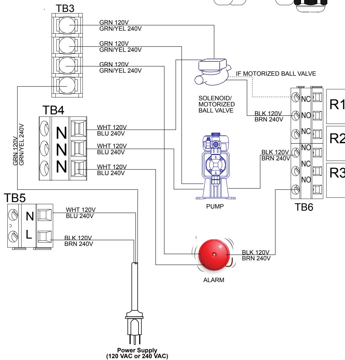
Figure 12 Digital Input /Analog Output Wiring
