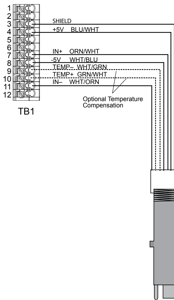
Figure 9 Non-Amplified pH/ORP/ISE Sensor Input Wiring pH/ORP/ISE ELECTRODE
