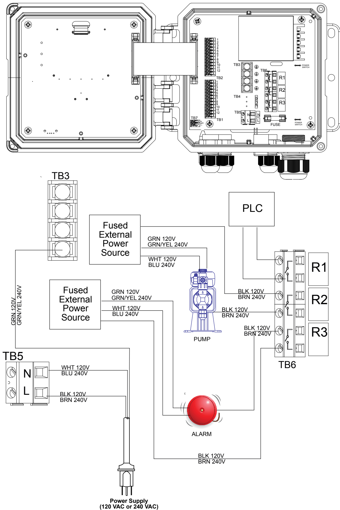
Figure 13 W100 AC Power & Relay Output Wiring
