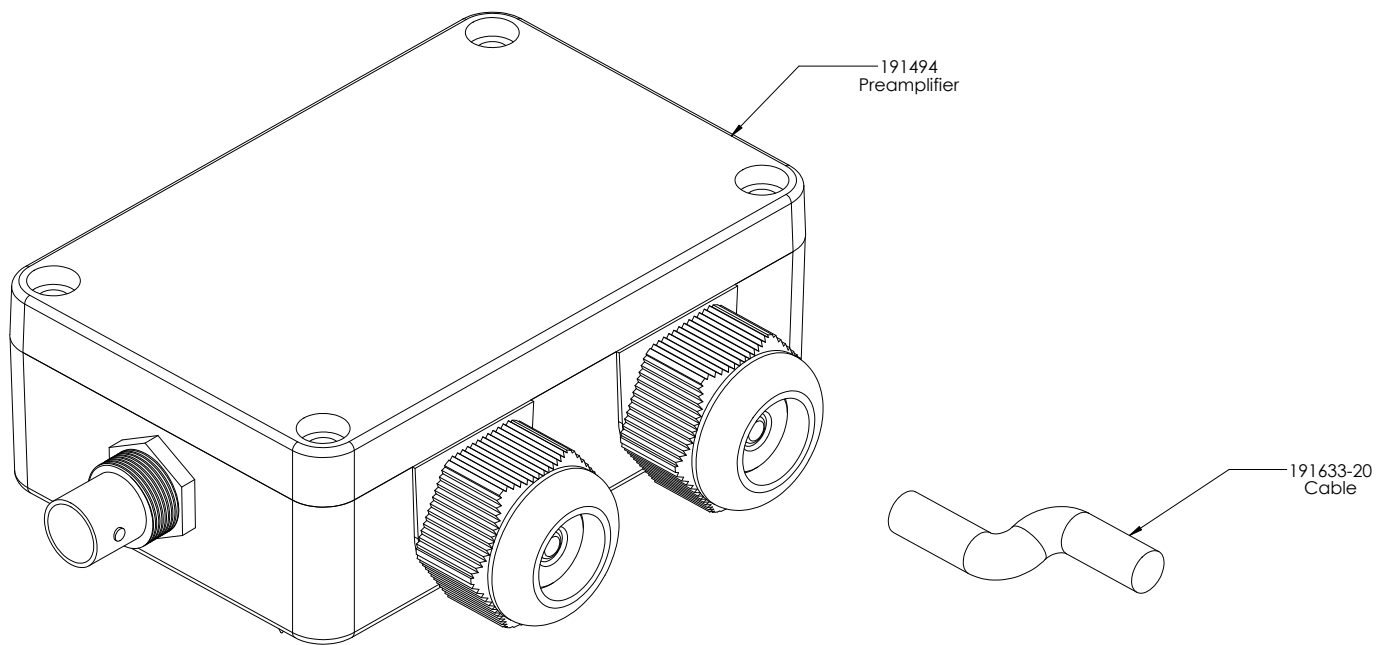
WPHPW Sensor Option A
