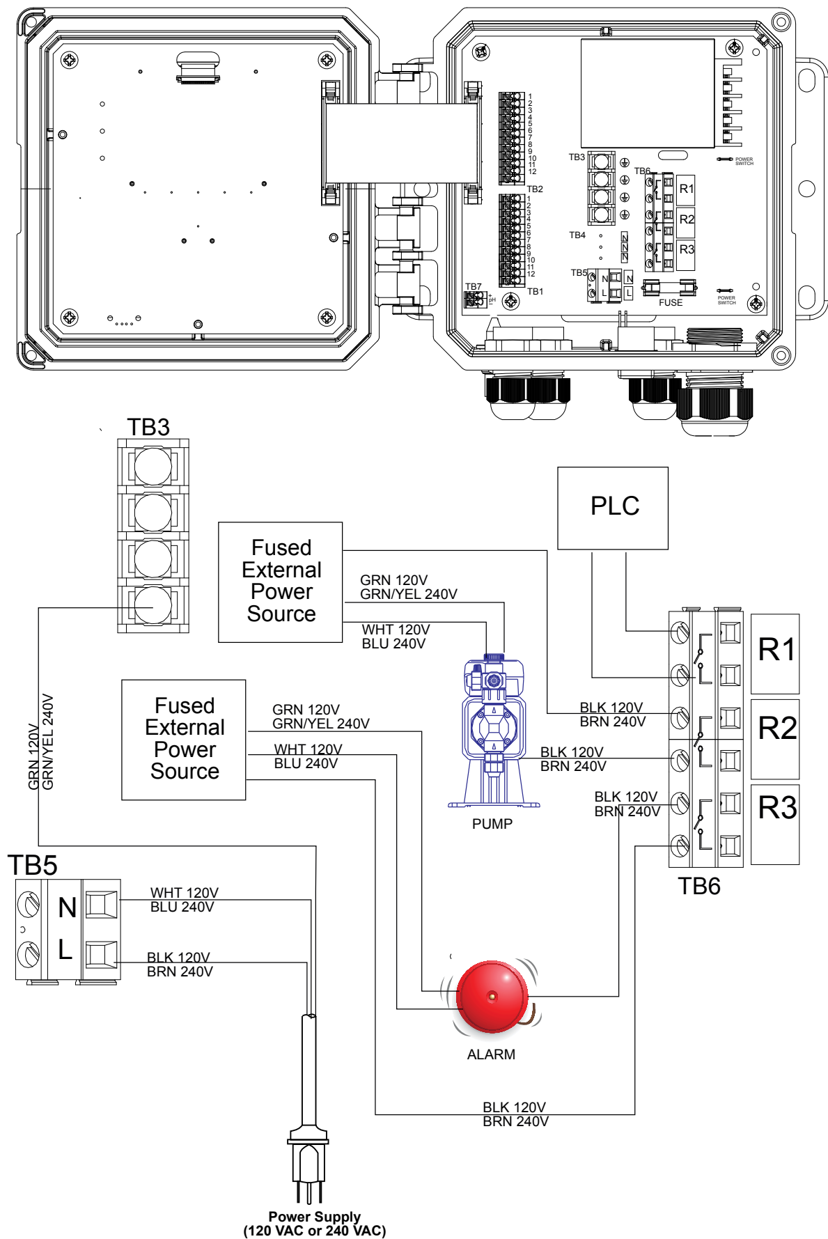
Figure 14 W110 AC Power & Relay Output Wiring
