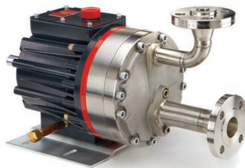
H25 with 316L Stainless Steel pump head and ANSI flanges.
