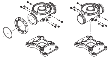
ANSI, PJE (Victaulic type)
