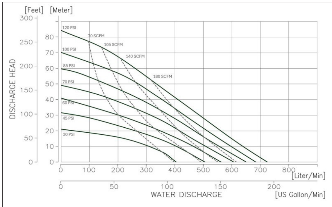
NDP-500 - PTFE Performance Curve
