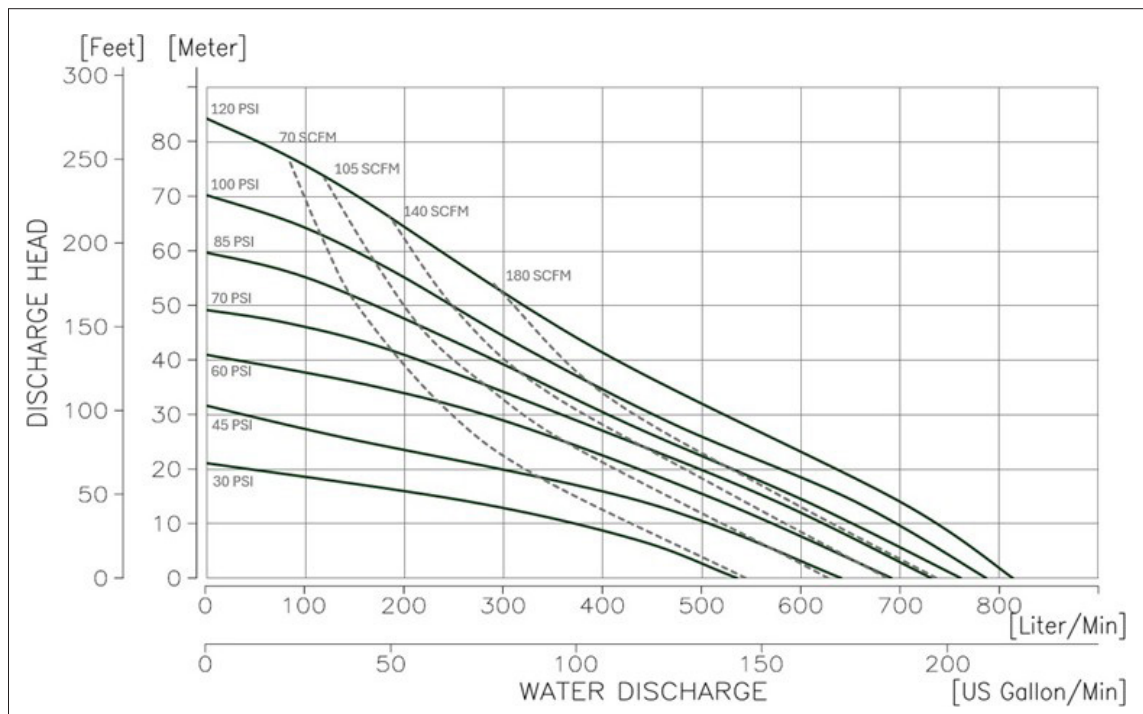
NDP-500 - Ultimate Performance Curve
