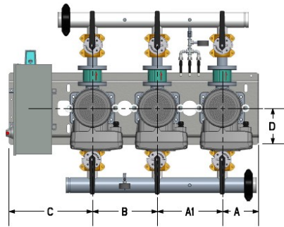
e-HVX Dimensions 10SVX Triplex Pump LEFT ORIENTATION
