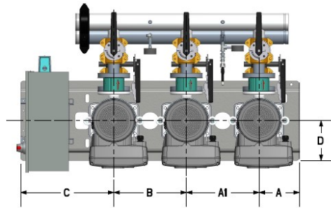
e-HVXR Dimensions 10SVX Triplex Pump LEFT ORIENTATION
